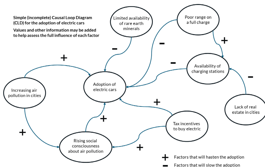
Figure 5: A partial Causal Loop Diagram
